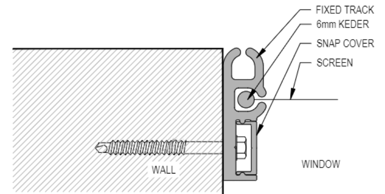
2 SECTION - INSIDE MOUNT SCALE: 12" = 1'-0"
